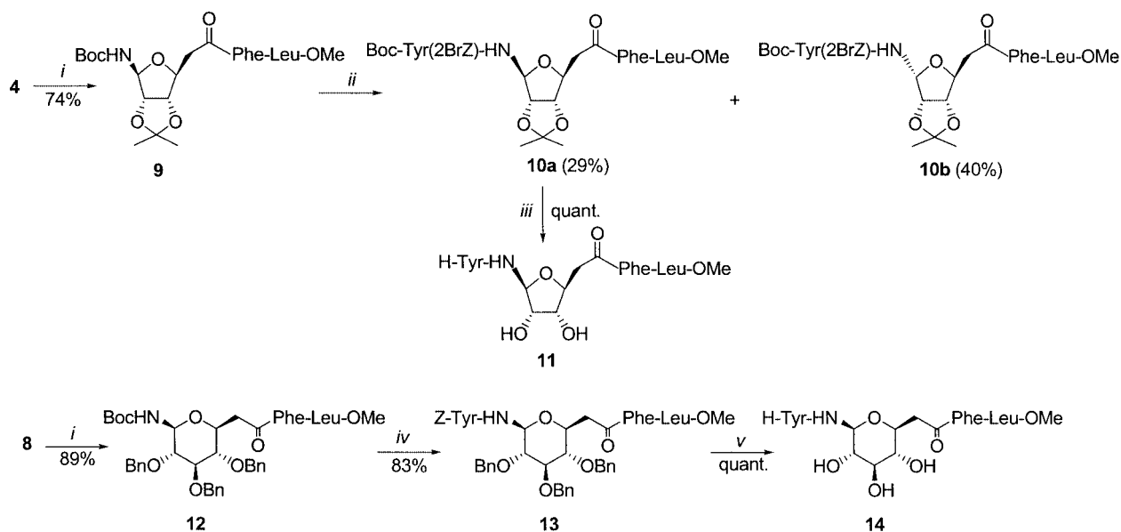
Scheme 3. Synthesis of Leu-enkephalin analogs 11 and 14 ; reagents and conditions: (i) HCl·H-Phe-Leu-OMe, EDC·HCl, HOBT, NMM, 16 h; (ii) a) 50%TFA/DCM, 5 min; b) Boc-Tyr(2BrZ)-OH, EDC·HCl, HOBT, NMM, 16 h; (iii) a) Pd(OH) 2 /C, MeOH, 5 h; b) 5% H 2 O/TFA, 3 h; (iv) a) 50%TFA/DCM, 5 min; b) Z-Tyr-OH, EDC·HCl, HOBT, NMM, 16 h; (v) Pd/C, H 2 , MeOH, 16 h
