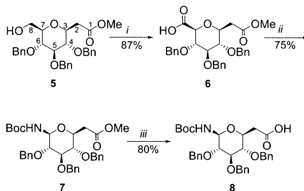
Scheme 2. Synthesis of pyranoid SAA; reagents and conditions: (i) PDC (10 equiv.), DMF, 16 h; (ii) DPPA, Et 3 N, t BuOH, 80 °C, 16 h; (iii) NaOH, dioxane, 3 h
