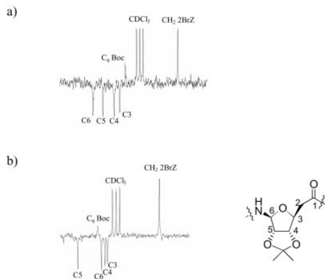
Figure 2. Parts of the 13 C NMR spectra of 10a (a) and 10b (b) recorded in CDCl 3 at 50 MHz
