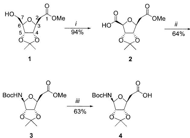
Scheme 1. Synthesis of furanoid SAA; reagents and conditions: (i) cat. TEMPO, NaOCl, NaHCO 3 , NaCl, KBr, ( n Bu) 4 NCl, DCM/H 2 O, 30 min, 0 °C; (ii) DPPA, Et 3 N, t BuOH, 80 °C, 16 h; (iii) LiOH, H 2 O 2 , THF, 0 °C, 2 h
